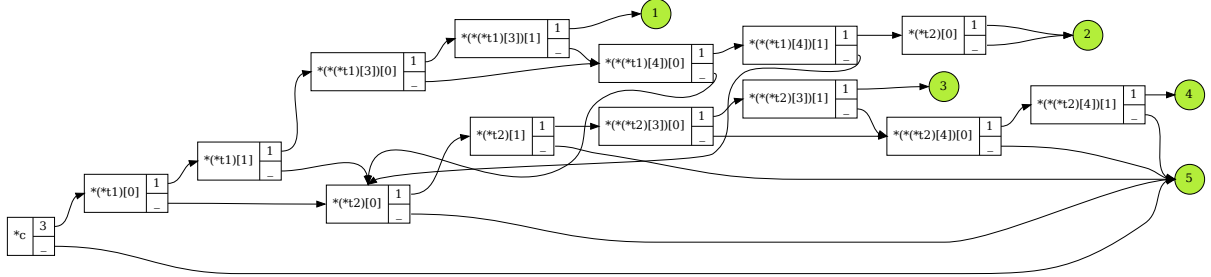
Figure 1: Example of Red-Black trees and their balancing operation in Rust
